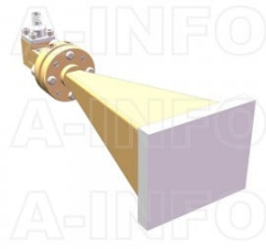
LB-10-25-C-1.0FSPO Standard Gain Horn Antenna 75-110GHz 25dB Gain 1.0mm Female
